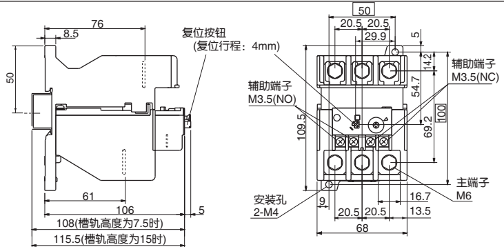
TR-N3H/3型, TR-N3HQ型 TK-N3H/3型, TK-N3HQ型
