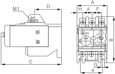
图2 JR20-10, 16, 25
