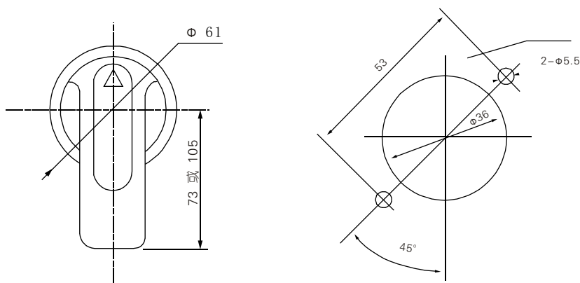
“A”型圆形手柄外形及门板开孔尺寸（开孔中心离铰链距离不小于100mm） Contour of model "A" round handle and the aperture dimension on the panel sheet (distance from the aperture center to hinge of panel door isn't less than 100mm)
