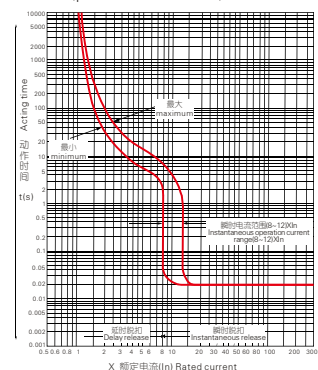
△ GSL1-100时间/电流特性曲线(配电) GSL1-100Time/Current characteristic curve(power distribution)
