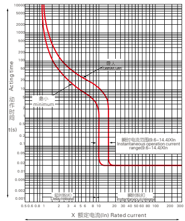
△ GSL1-100时间/电流特性曲线 (电动机) GSL1-100Time/Current characteristic curve (power distribution)
