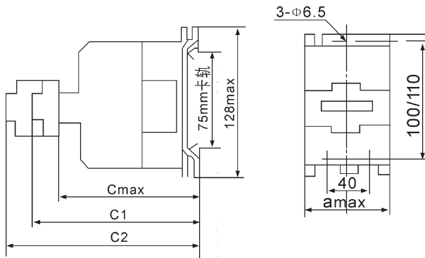
△ GSC1-4004/9504外形及安装尺寸图 Outline dimension and mounting dimensions
