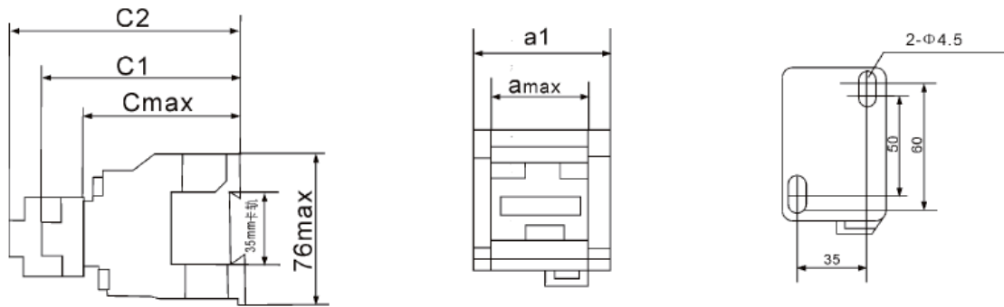
△ GSC1-0904/1204外形及安装尺寸图 Outline dimension and mounting dimensions
