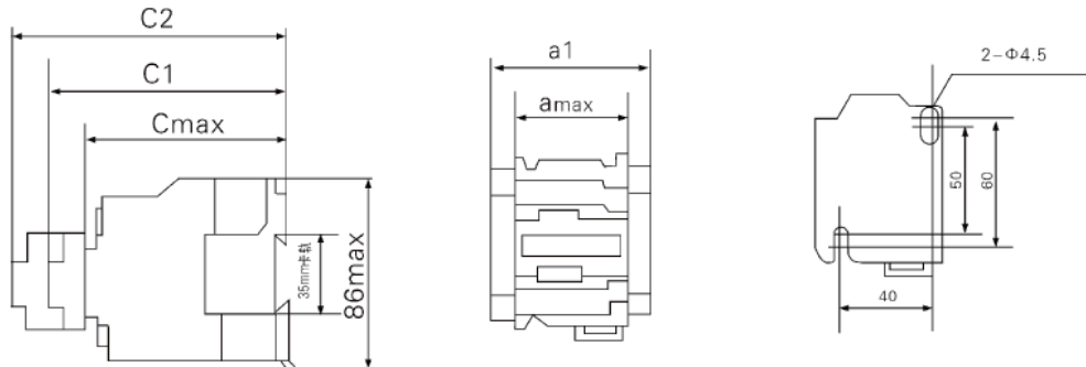
△ GSC1-1804/2504外形及安装尺寸图 Outline dimension and mounting dimensions
