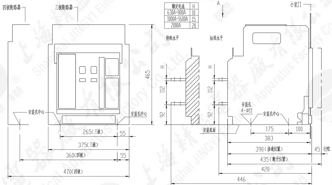
HA1-2000 630A~2000A 3P/4P 抽屉式断路器 (Draw-out ACB)
