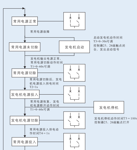
电网-发电机型自投自复功能逻辑图
