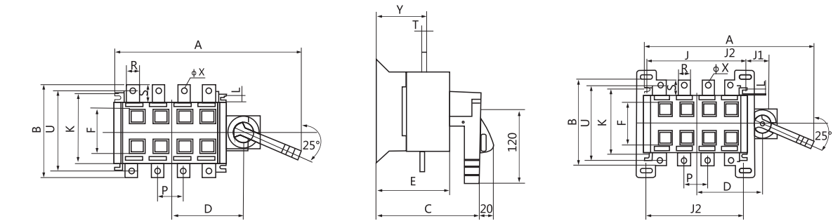
RDH5(HGL)C-125~630A/K
