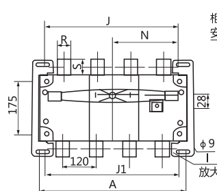
RDH5(HGL)-1000A ~ 1600A/J
