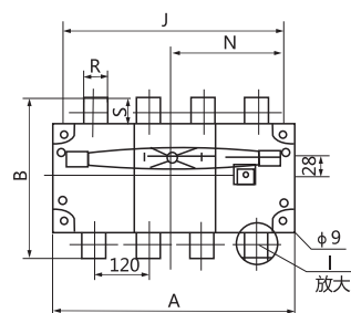
RDH5(HGL)-1000A ~ 1600A
